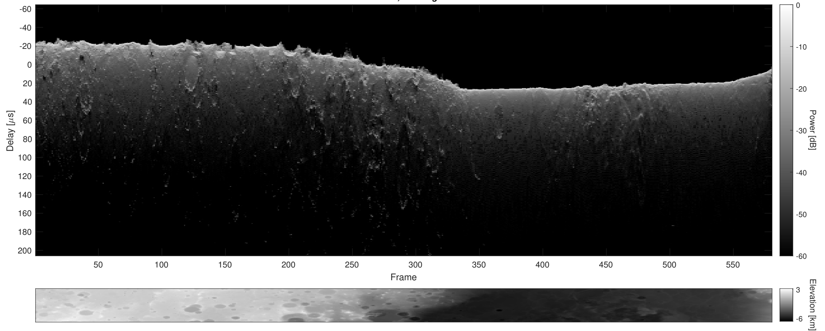
Orbit 4798, Cluttergram
