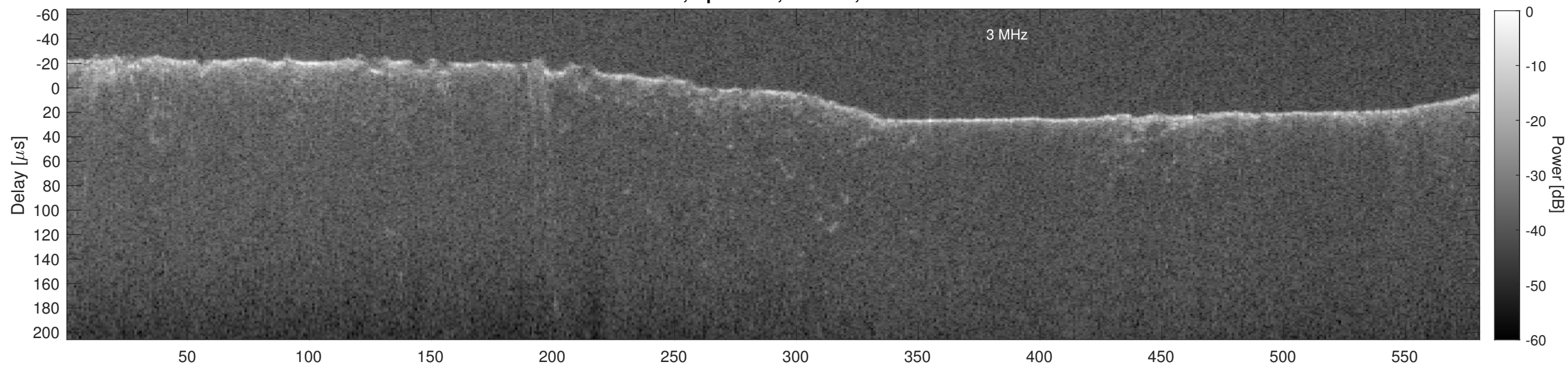
Orbit 4798, Cluttergram
