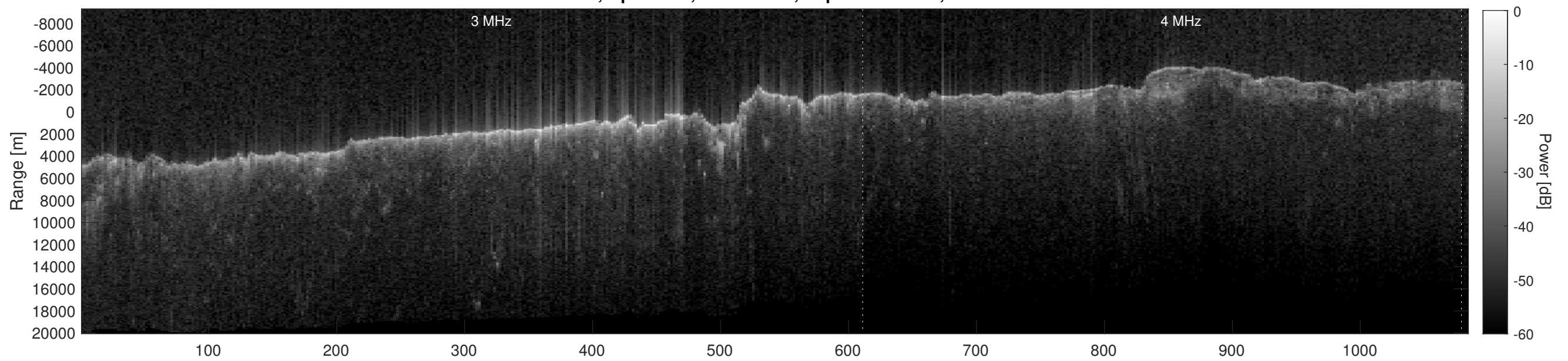
Orbit 4799, Depth-Corrected Cluttergram
