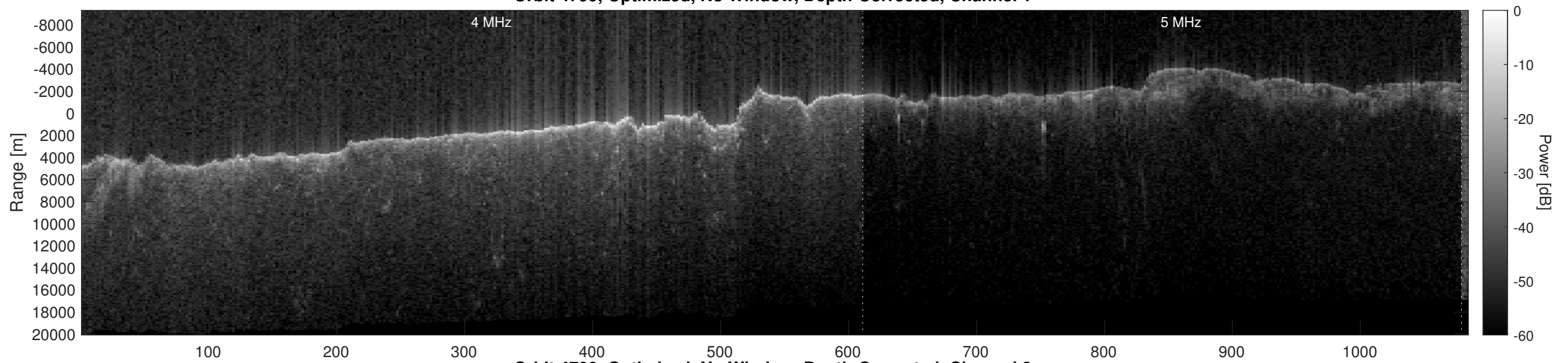
Orbit 4799, Optimized, No Window, Depth-Corrected, Channel 2
