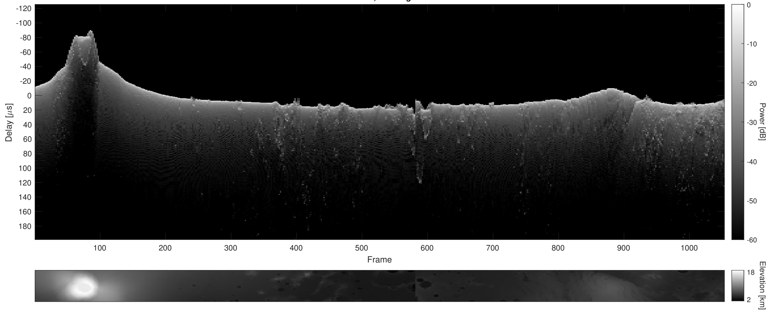
Orbit 4800, Cluttergram
