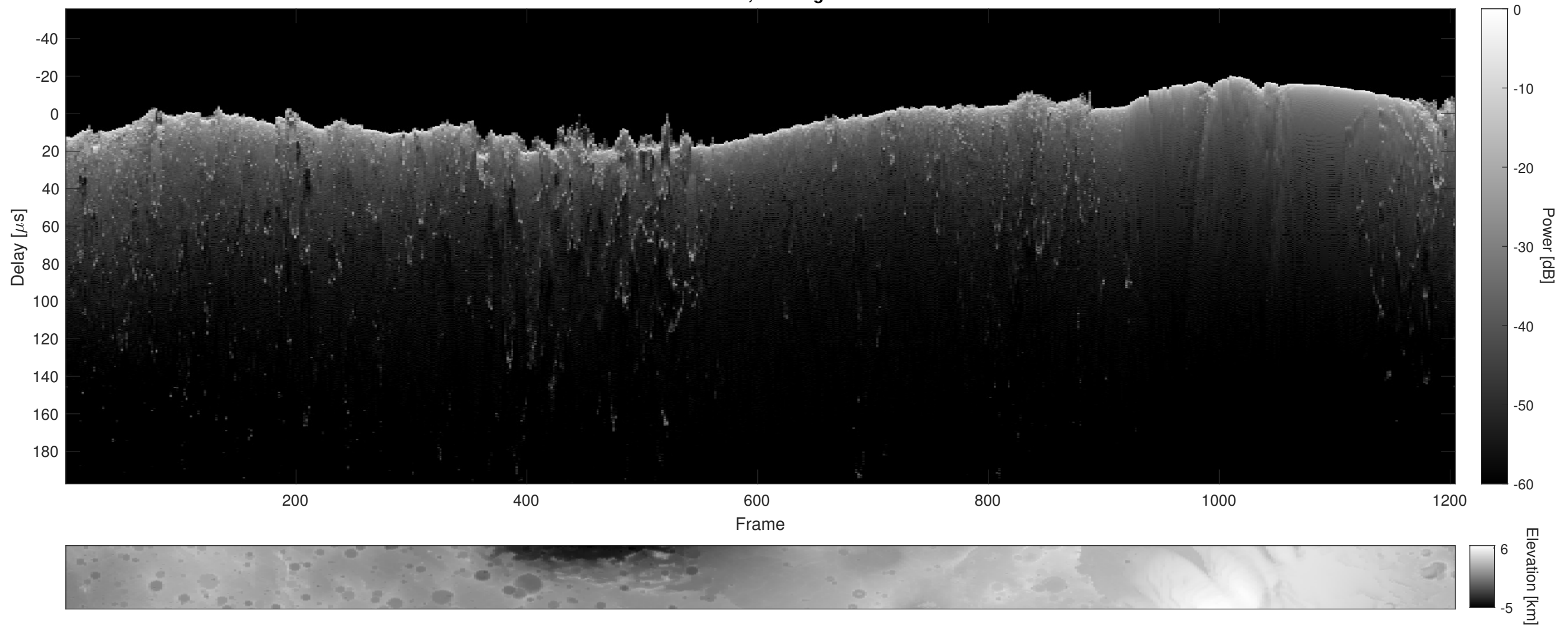
Orbit 4802, Cluttergram
