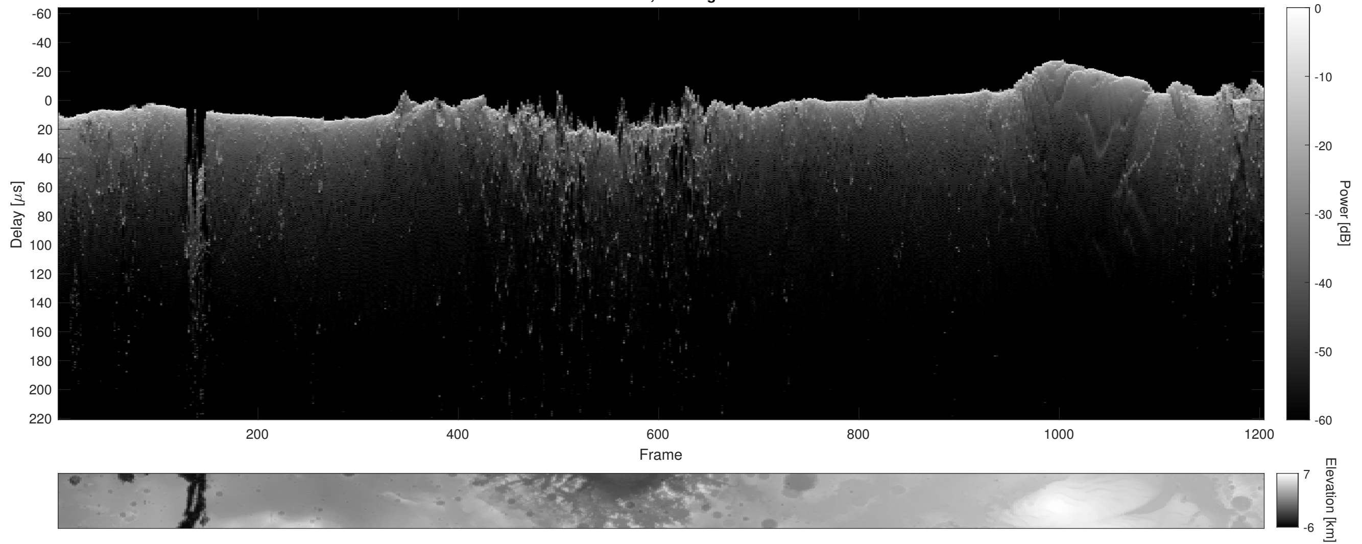
Orbit 4803, Cluttergram
