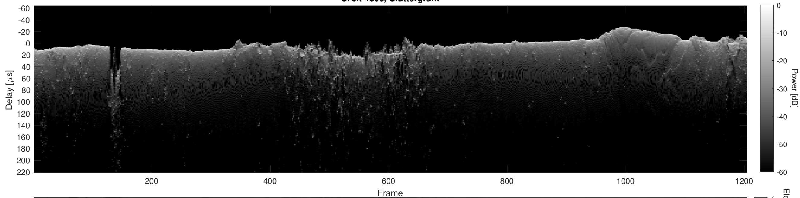
Orbit 4803, Cluttergram
