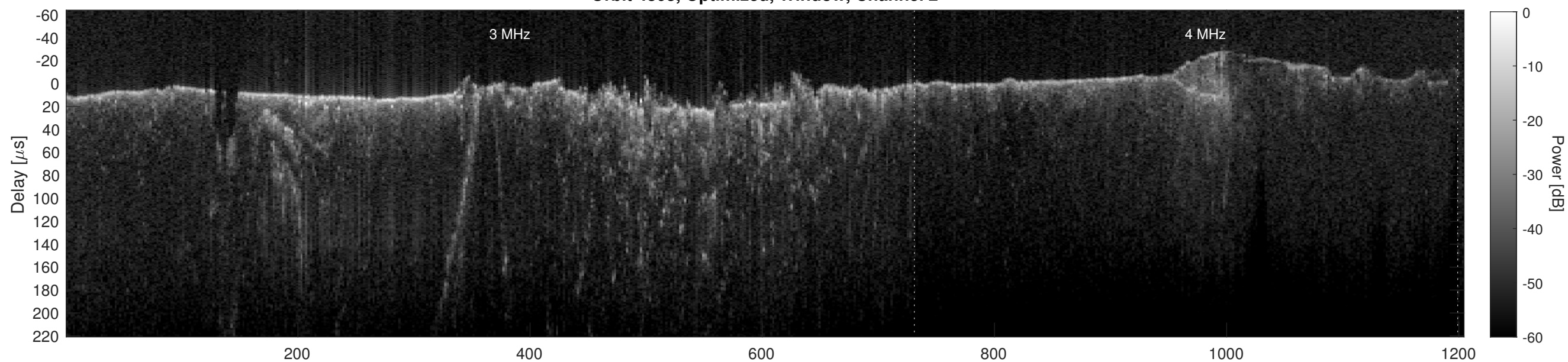
Orbit 4803, Cluttergram
