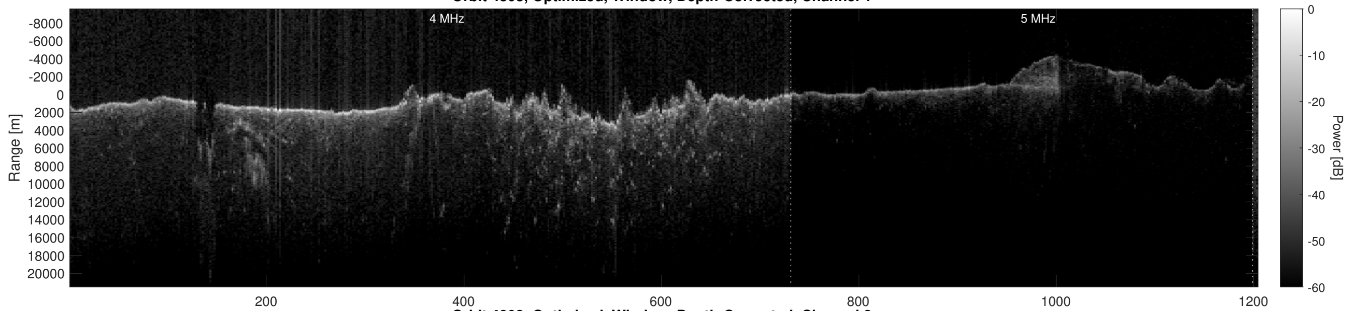
Orbit 4803, Optimized, Window, Depth-Corrected, Channel 2
