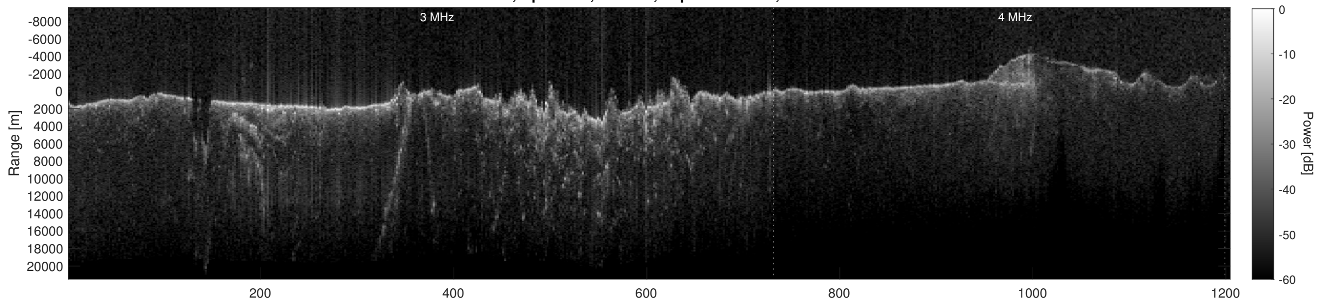
Orbit 4803, Depth-Corrected Cluttergram
