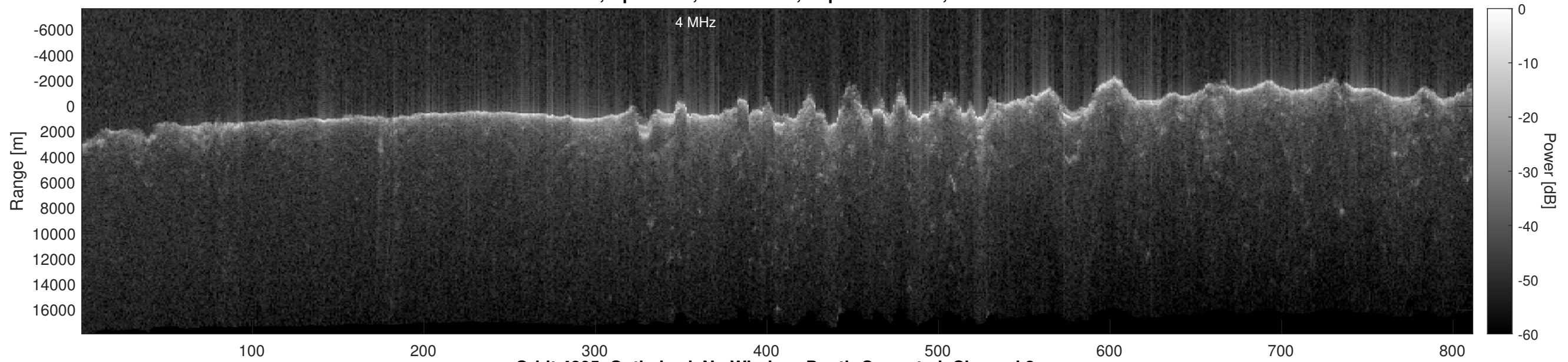
Orbit 4805, Optimized, No Window, Depth-Corrected, Channel 2
