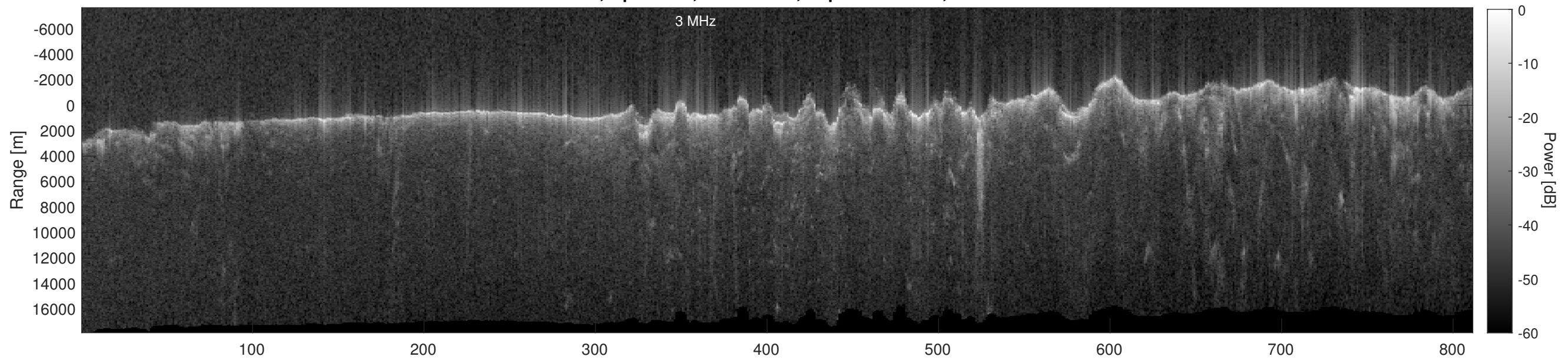
Orbit 4805, Depth-Corrected Cluttergram
