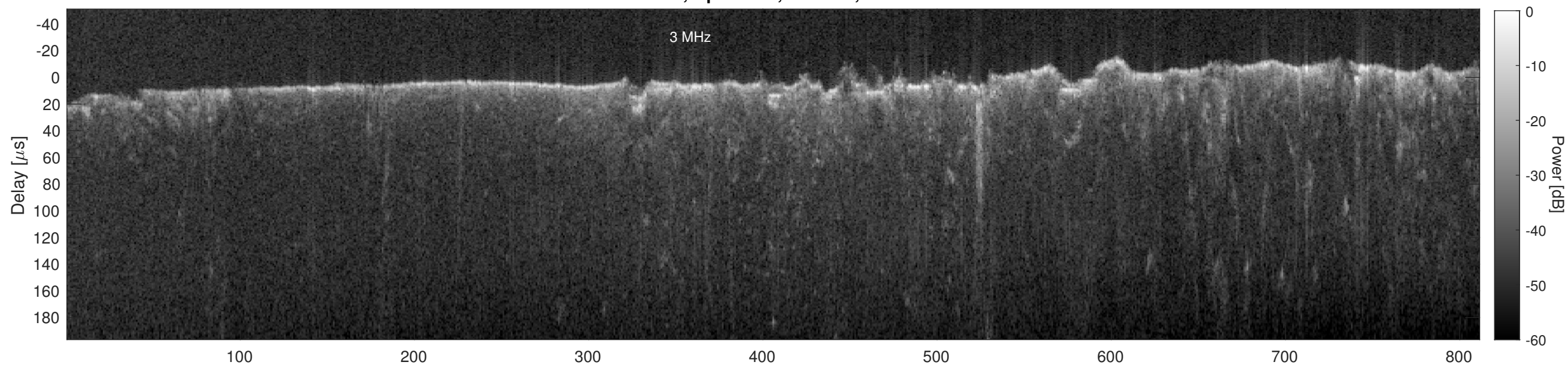
Orbit 4805, Cluttergram
