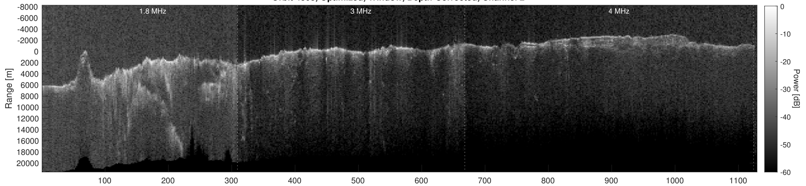
Orbit 4808, Depth-Corrected Cluttergram
