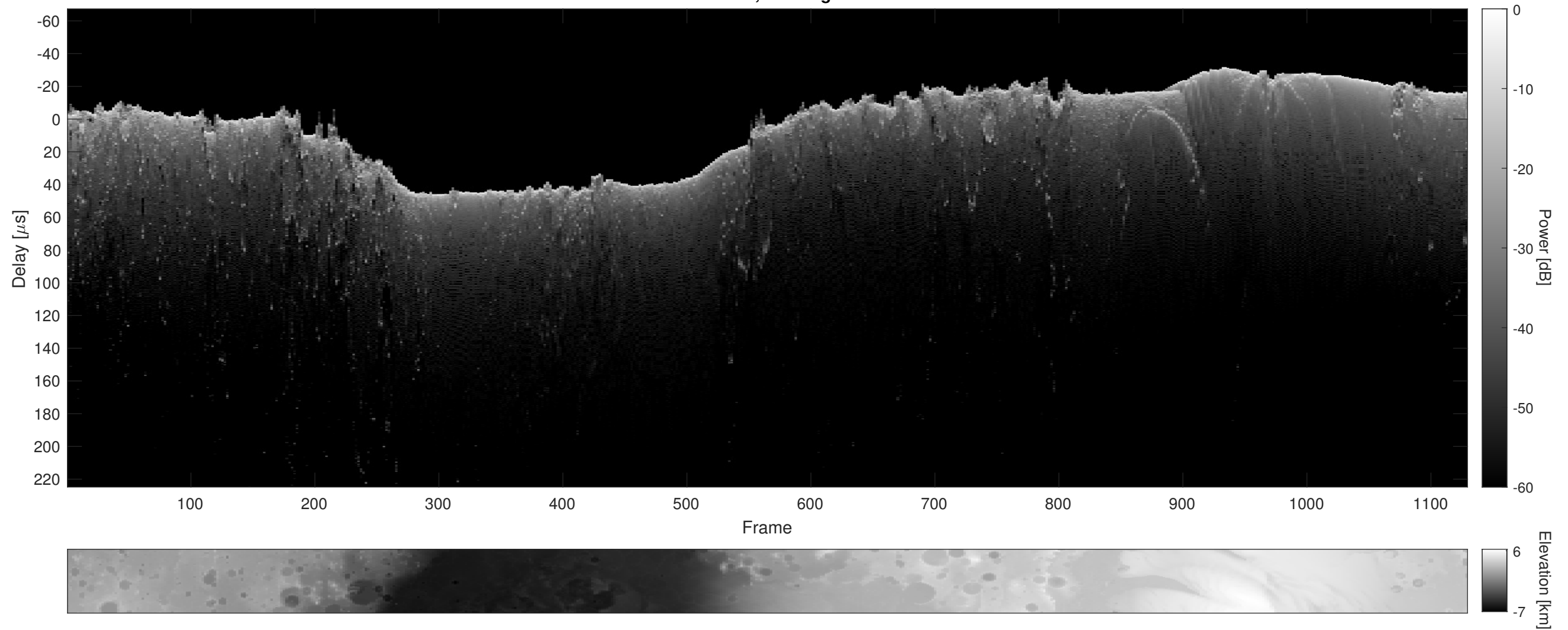
Orbit 4809, Cluttergram
