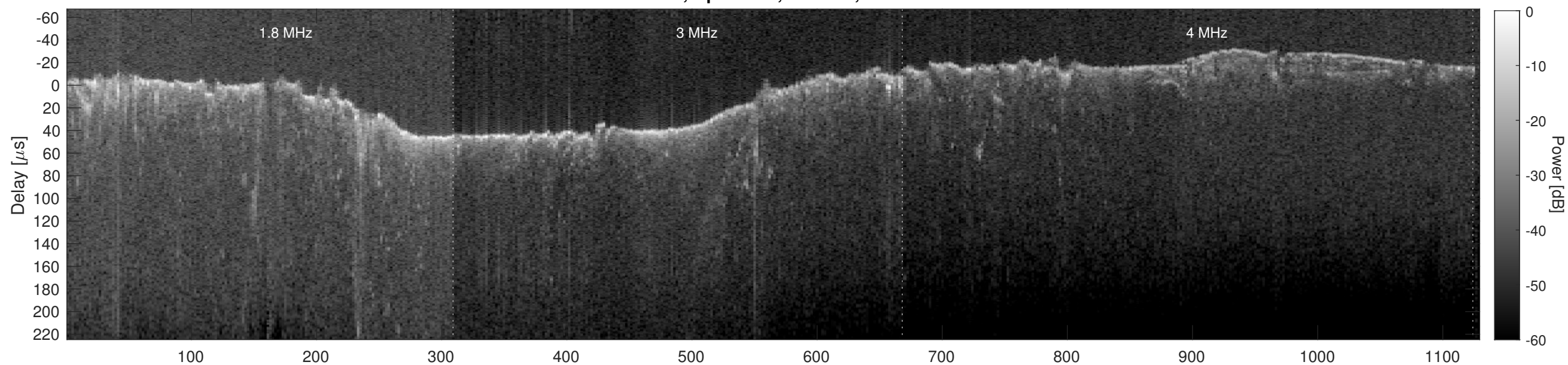
Orbit 4809, Cluttergram
