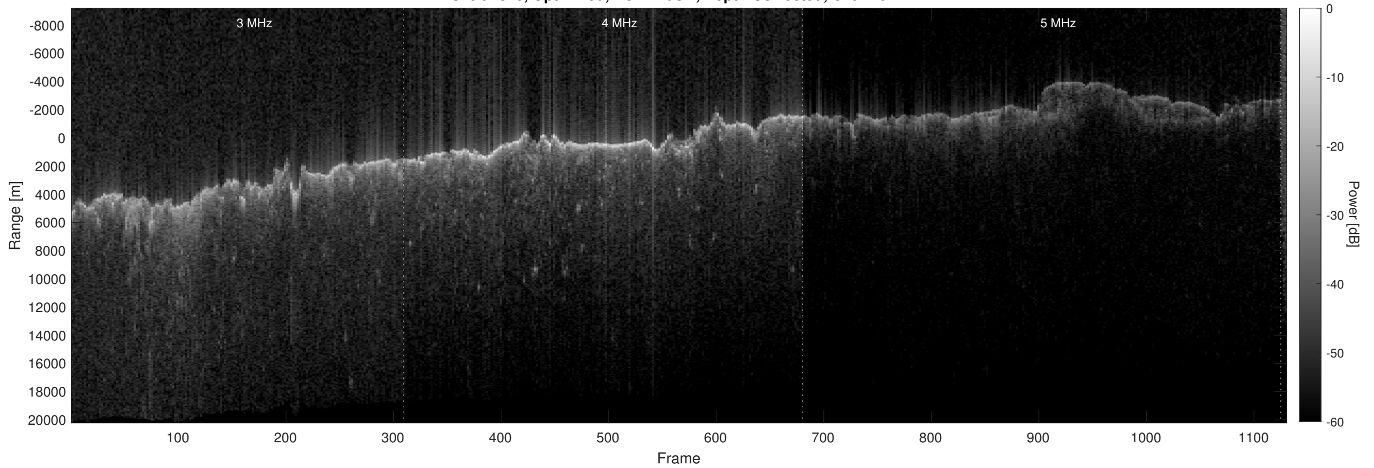
Orbit 4810, Optimized, No Window, Depth-Corrected, Channel 2
