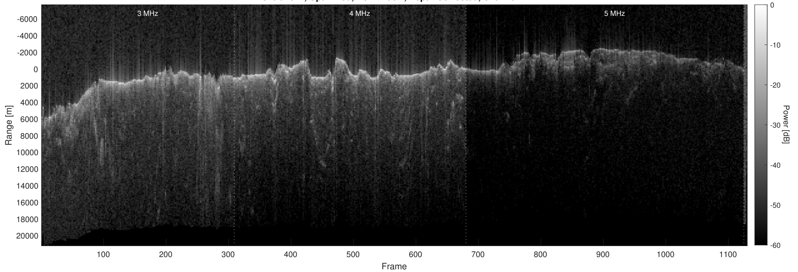
Orbit 4812, Optimized, No Window, Depth-Corrected, Channel 2
