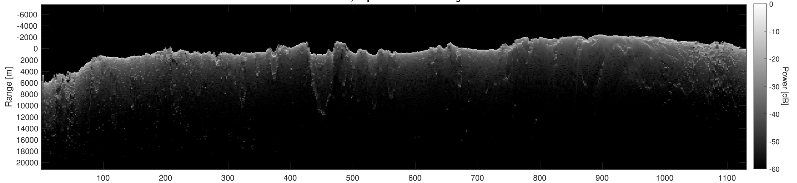
Orbit 4812, Depth-Corrected Cluttergram
