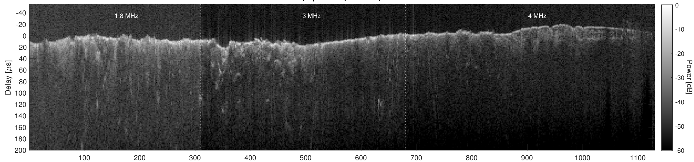
Orbit 4813, Cluttergram
