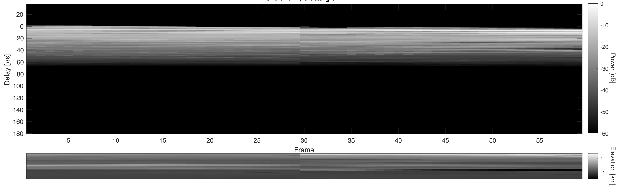
Orbit 4814, Cluttergram
