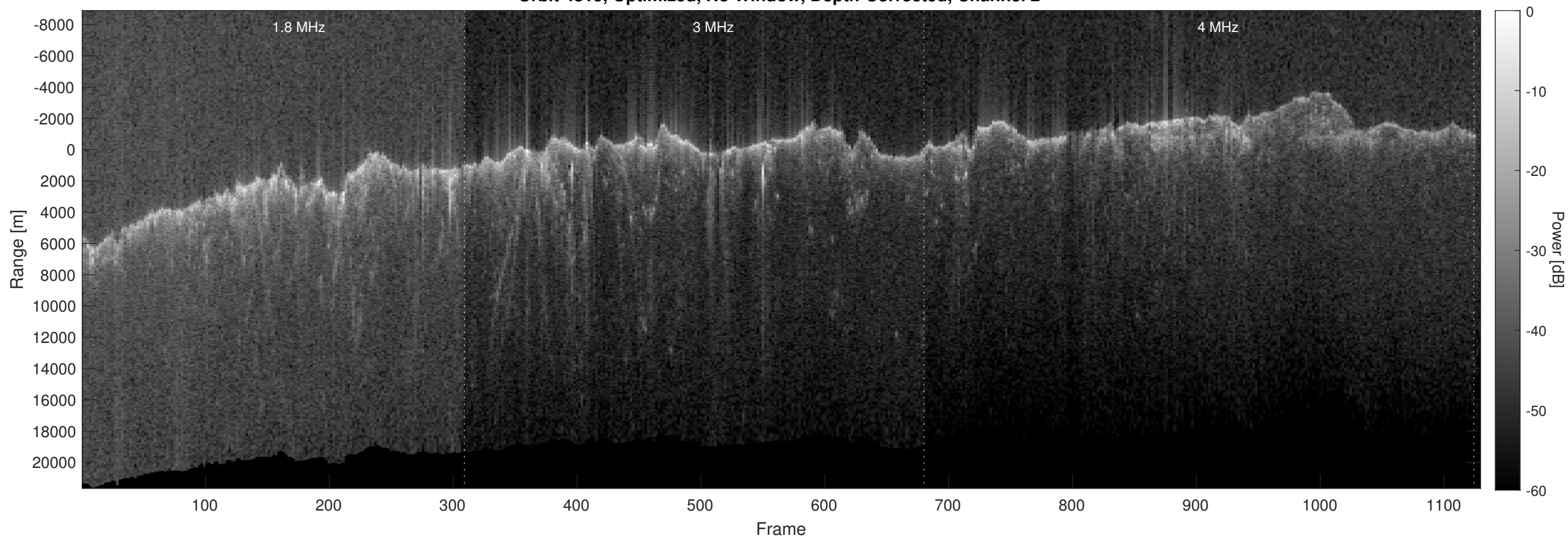
Orbit 4815, Optimized, No Window, Depth-Corrected, Channel 2
