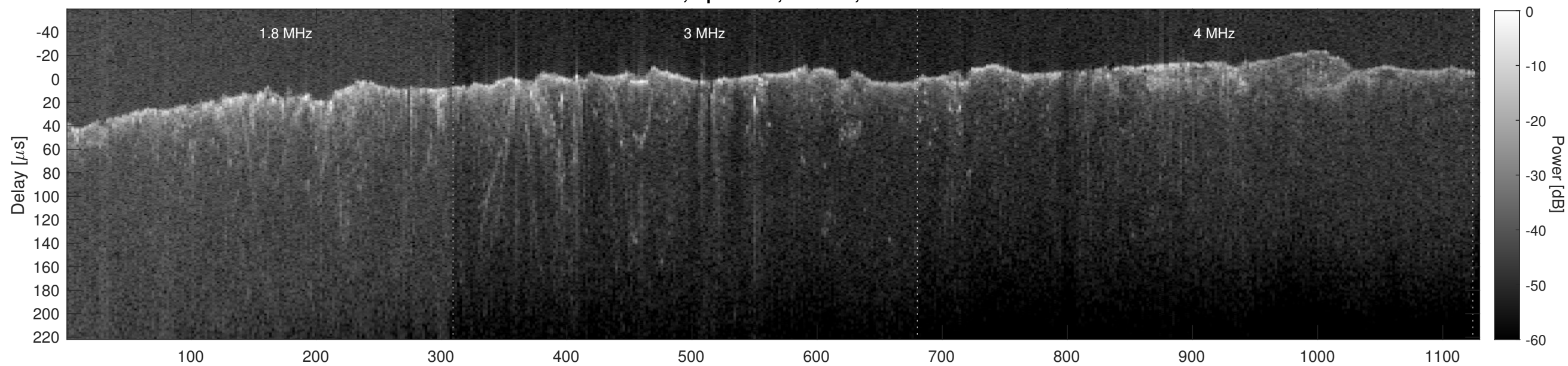
Orbit 4815, Cluttergram
