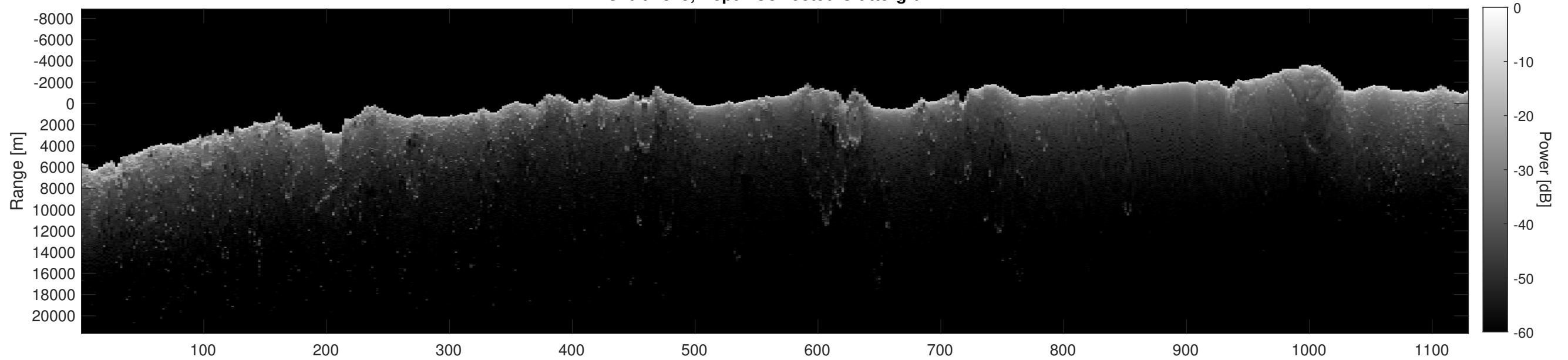
Orbit 4815, Depth-Corrected Cluttergram
