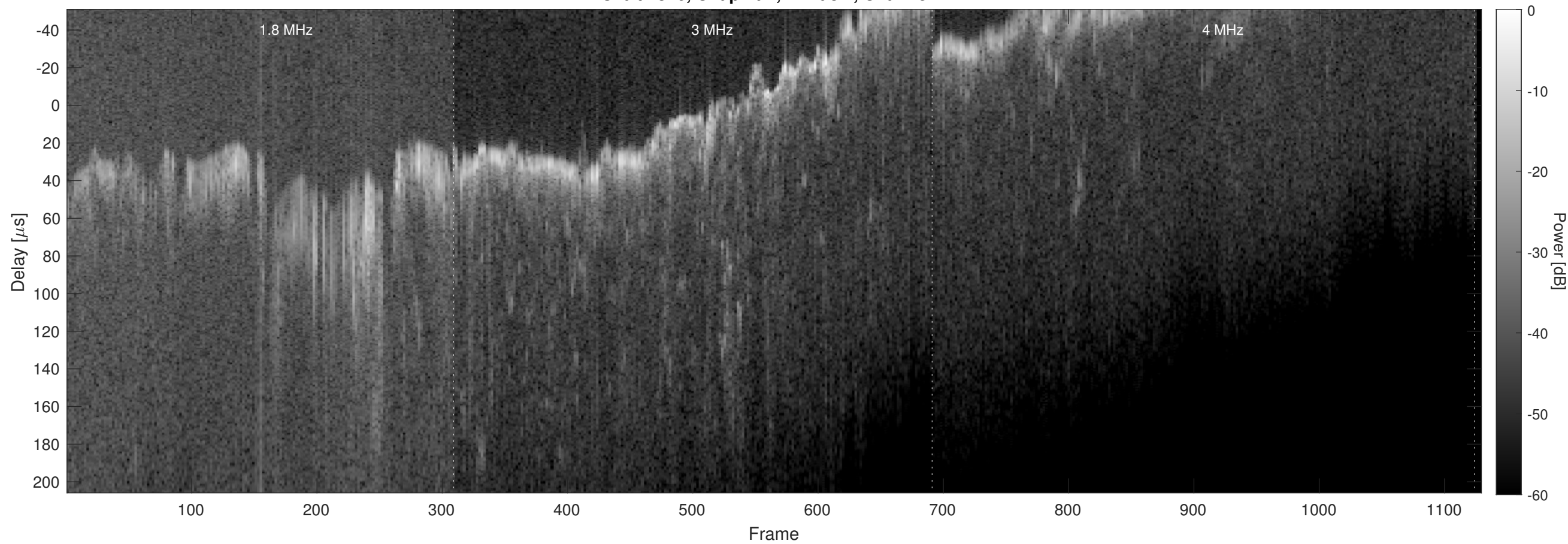
Orbit 4816, Chapman, Window, Channel 2
