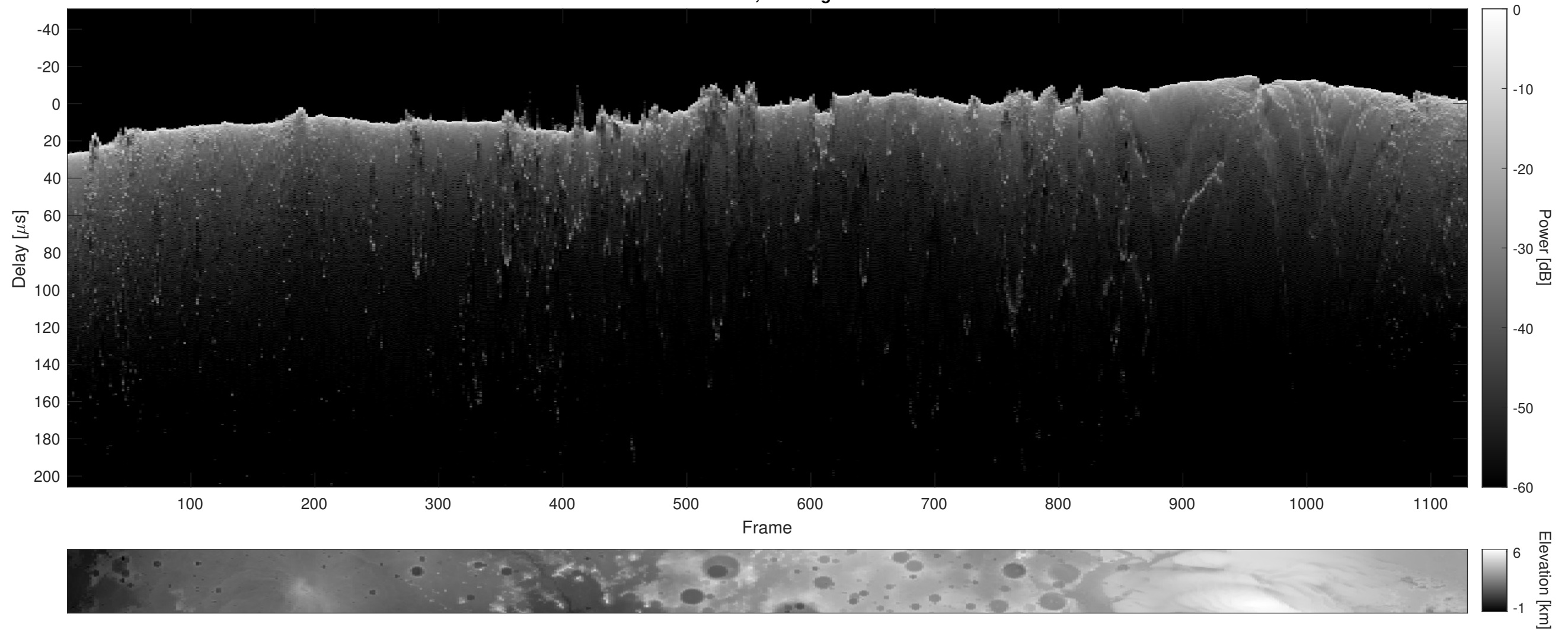
Orbit 4816, Cluttergram
