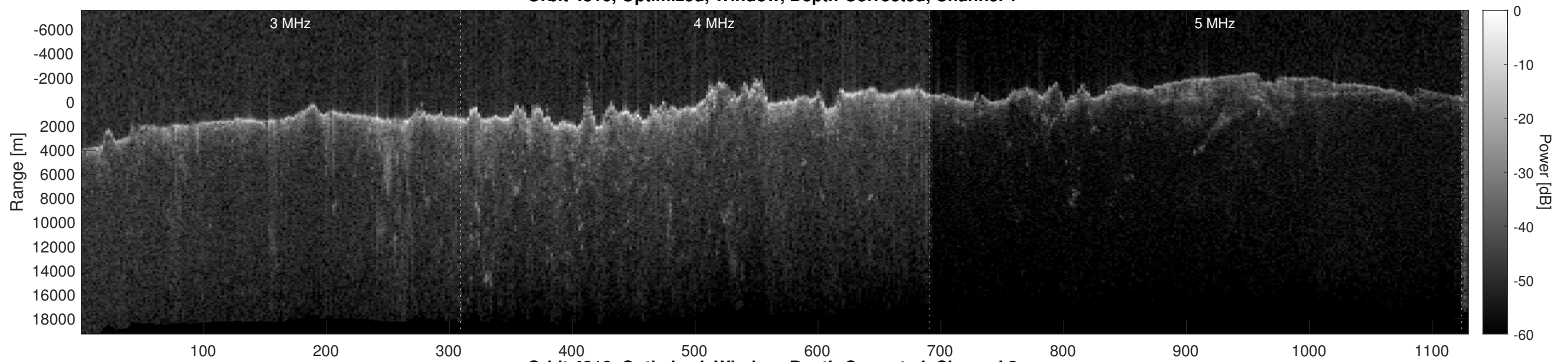
Orbit 4816, Optimized, Window, Depth-Corrected, Channel 2
