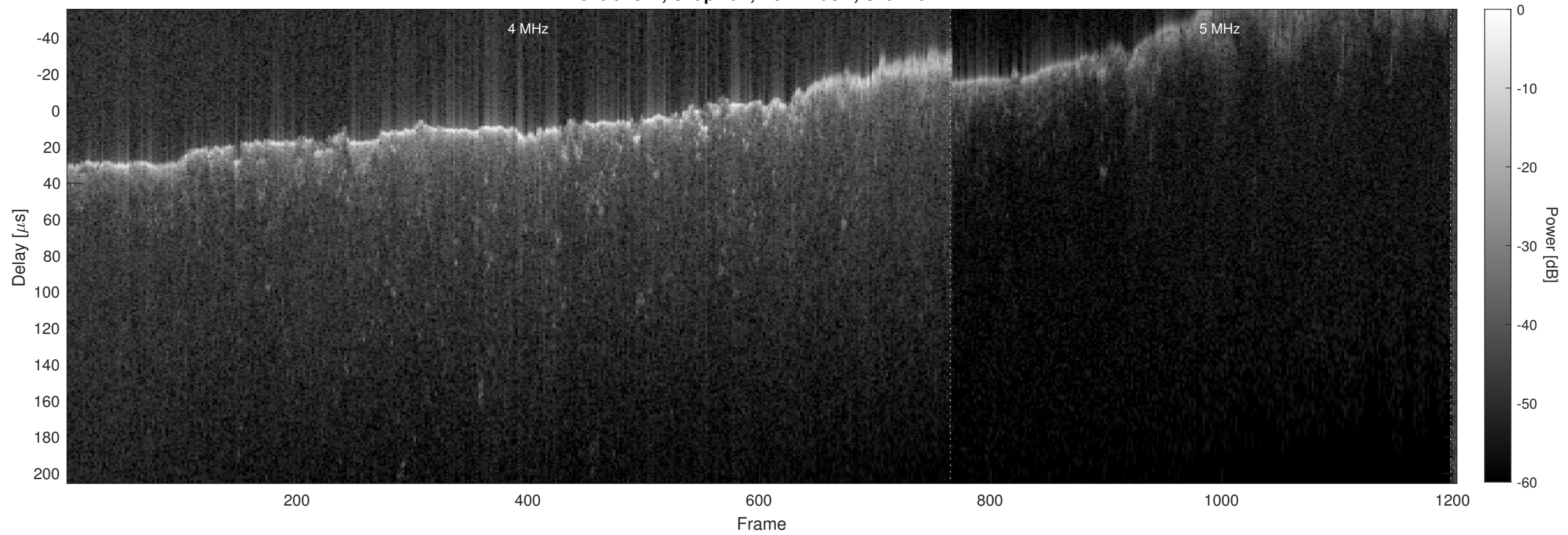
Orbit 4817, Chapman, No Window, Channel 2
