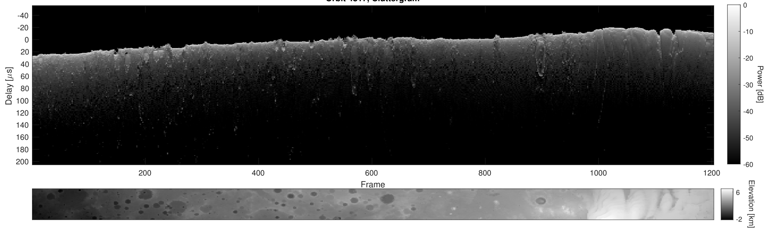
Orbit 4817, Cluttergram
