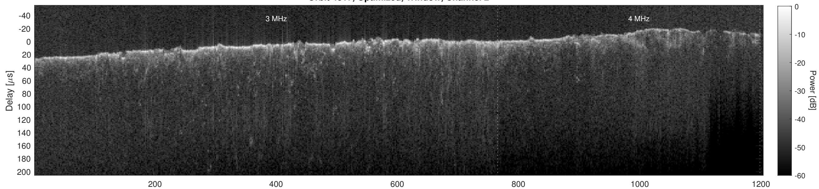
Orbit 4817, Cluttergram
