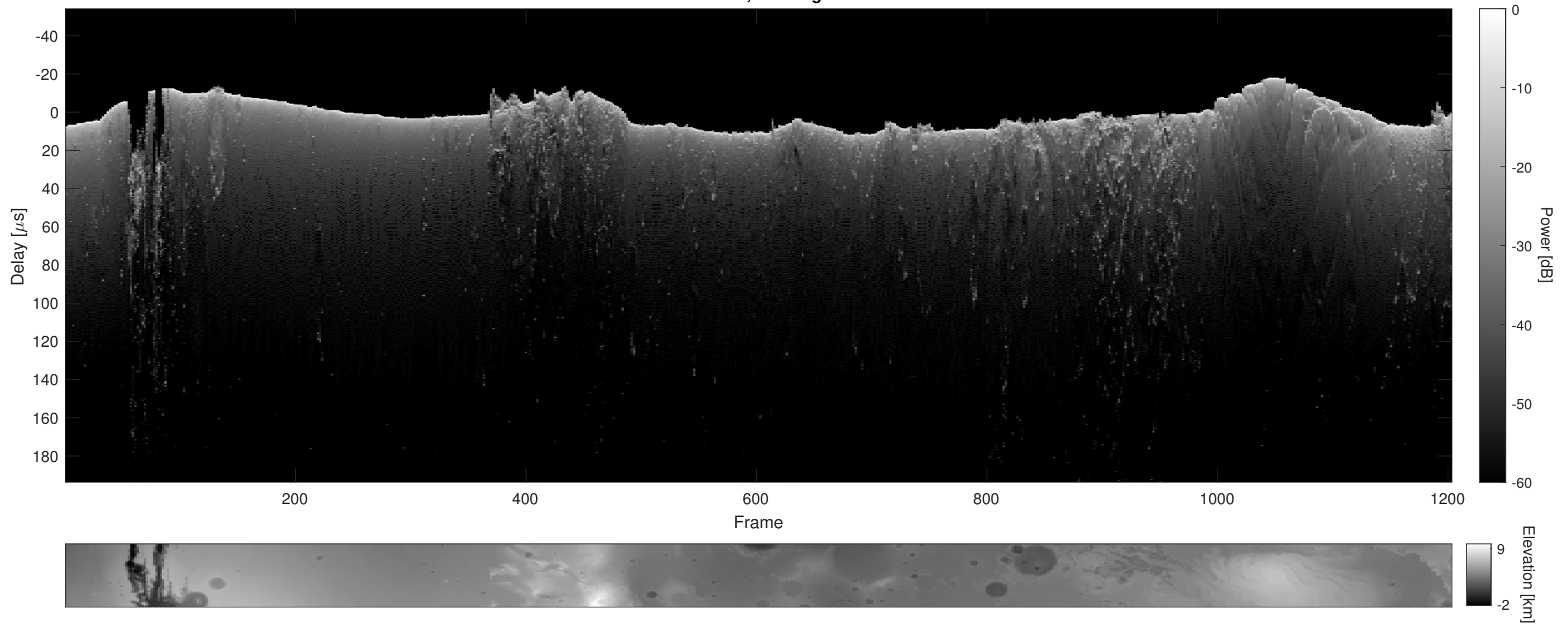
Orbit 4818, Cluttergram
