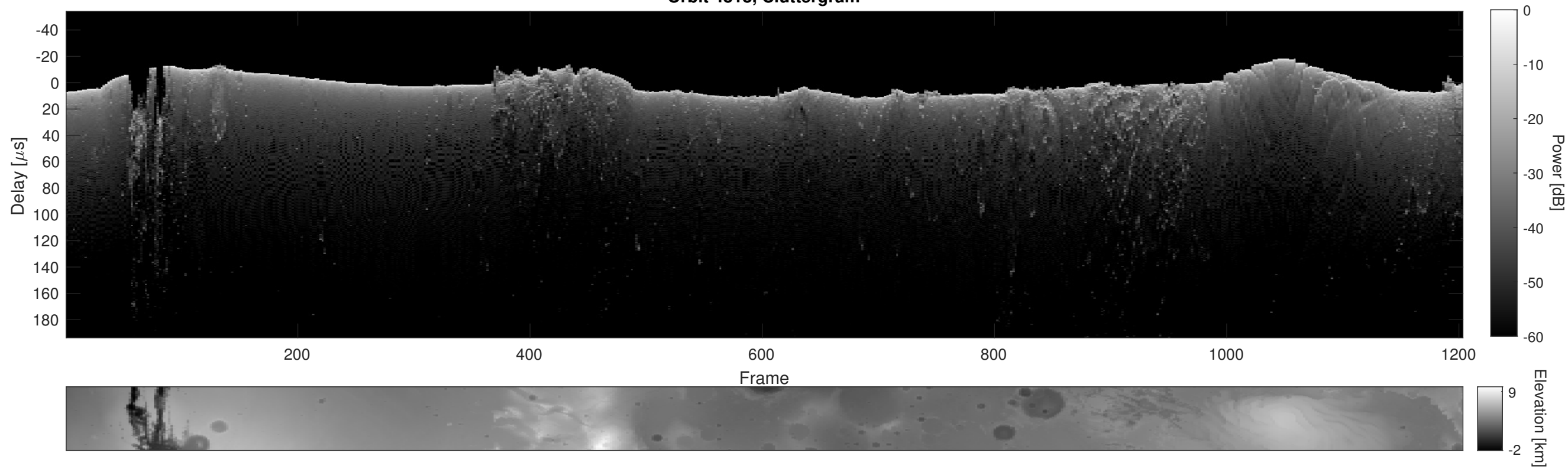
Orbit 4818, Cluttergram
