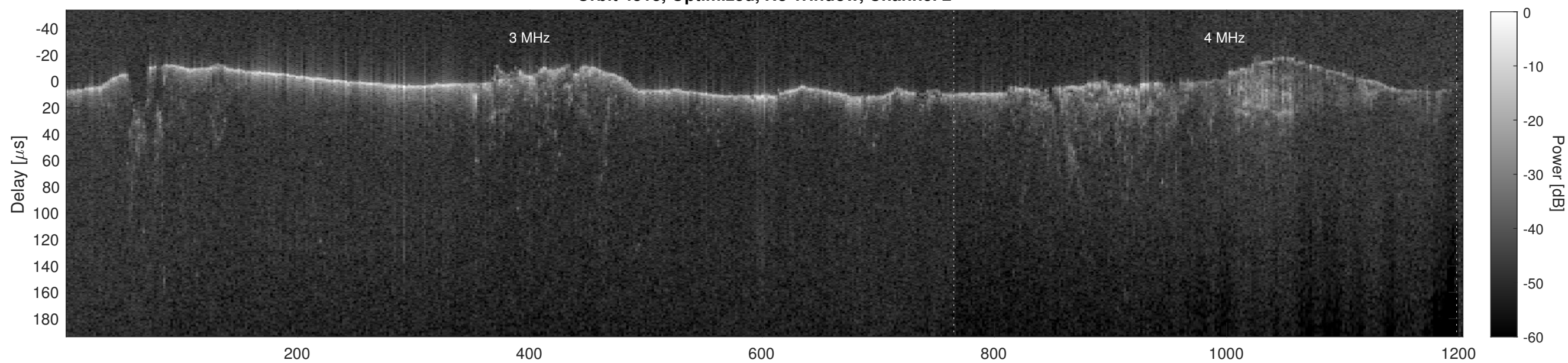
Orbit 4818, Cluttergram
