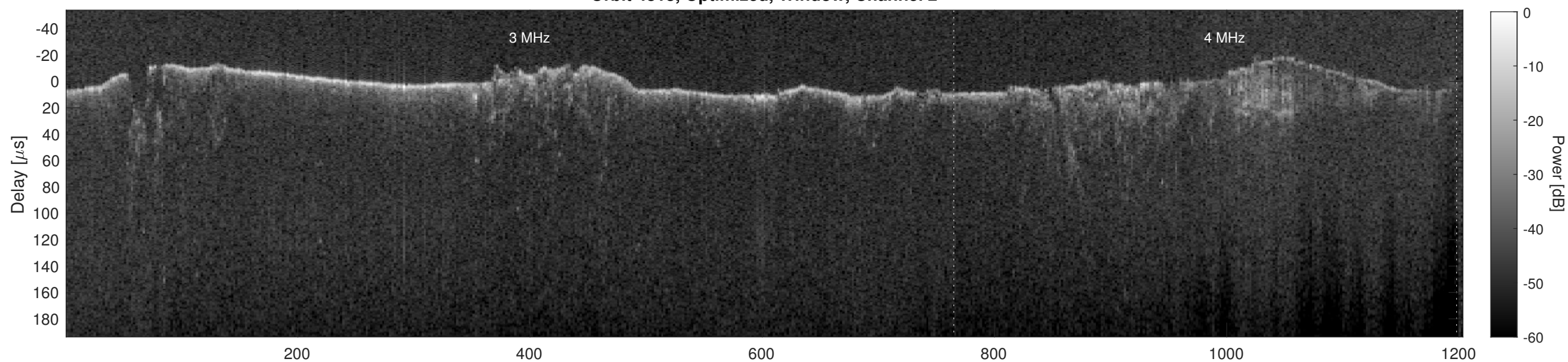
Orbit 4818, Cluttergram
