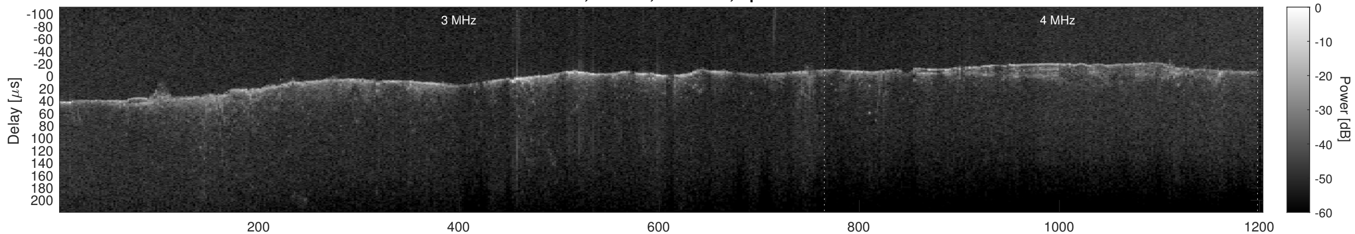
Orbit 4819, Cluttergram
