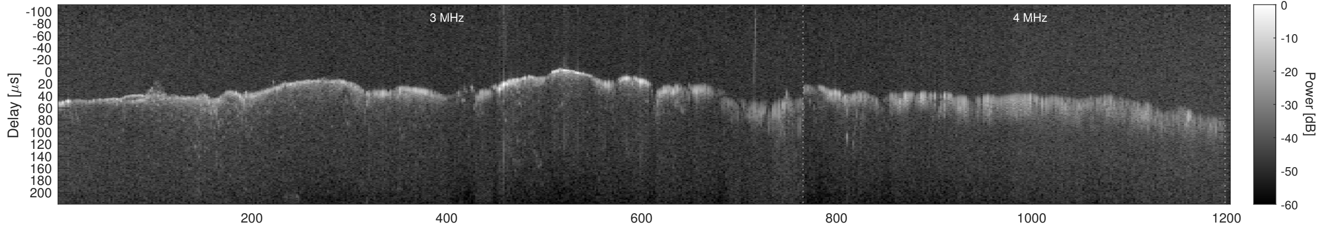
Orbit 4819, Window, Channel 2, Chapman
