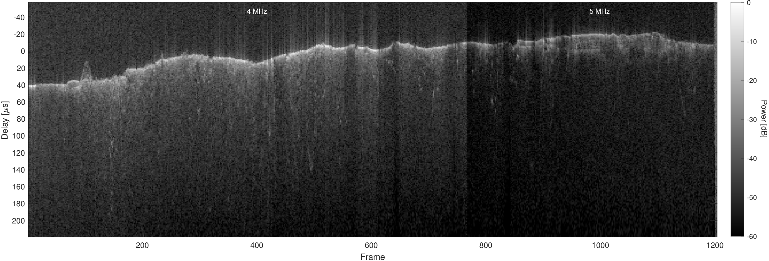
Orbit 4819, Optimized, No Window, Channel 2
