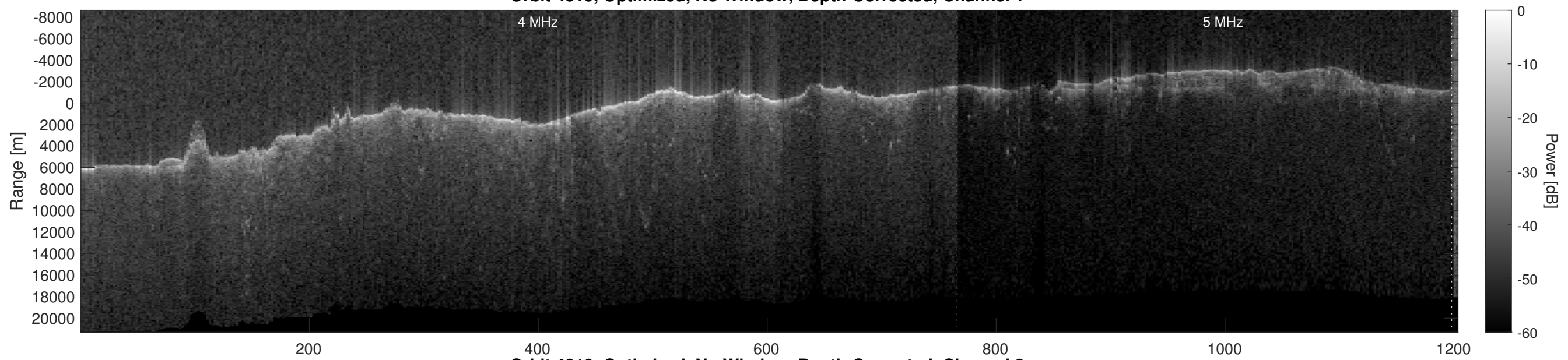
Orbit 4819, Optimized, No Window, Depth-Corrected, Channel 2
