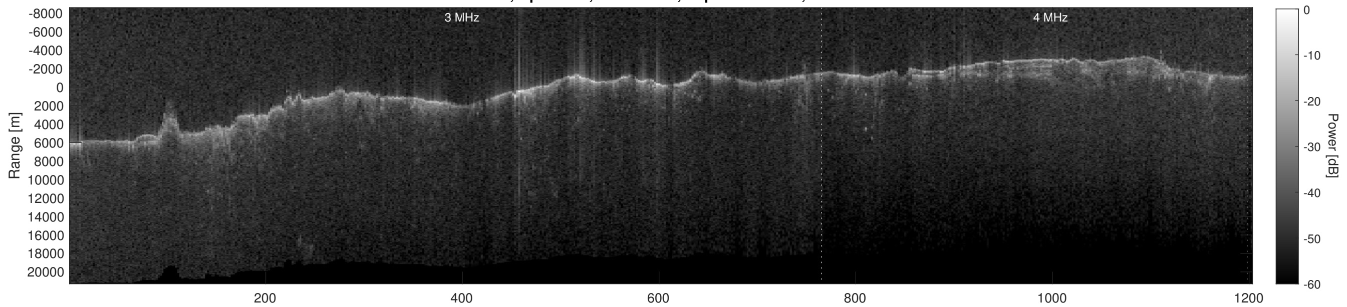
Orbit 4819, Depth-Corrected Cluttergram
