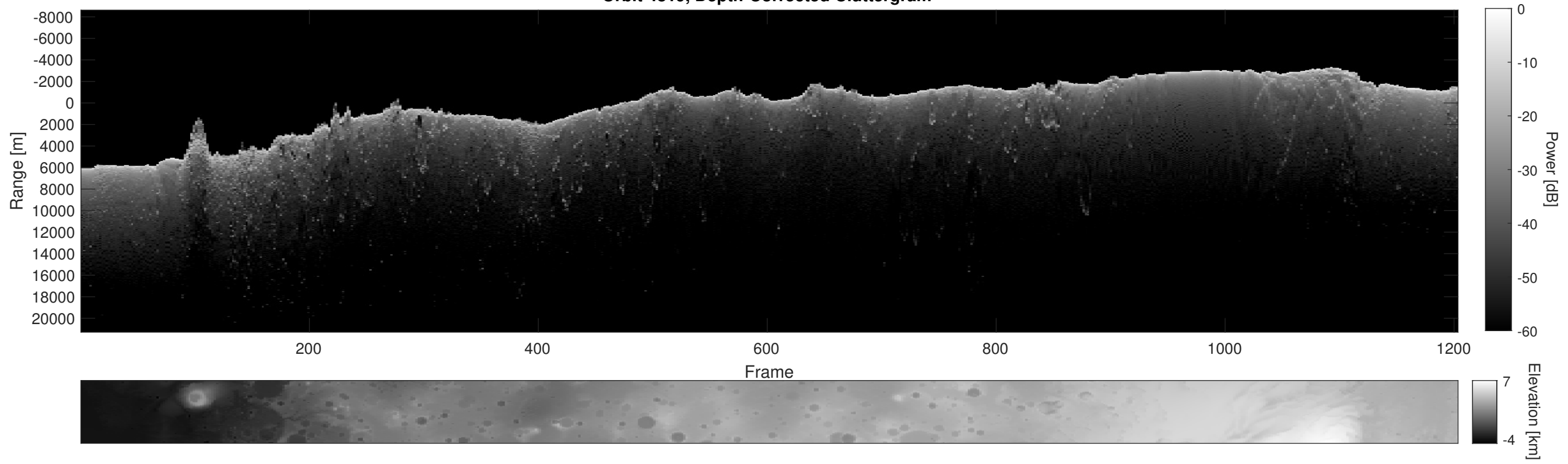
Orbit 4819, Depth-Corrected Cluttergram
