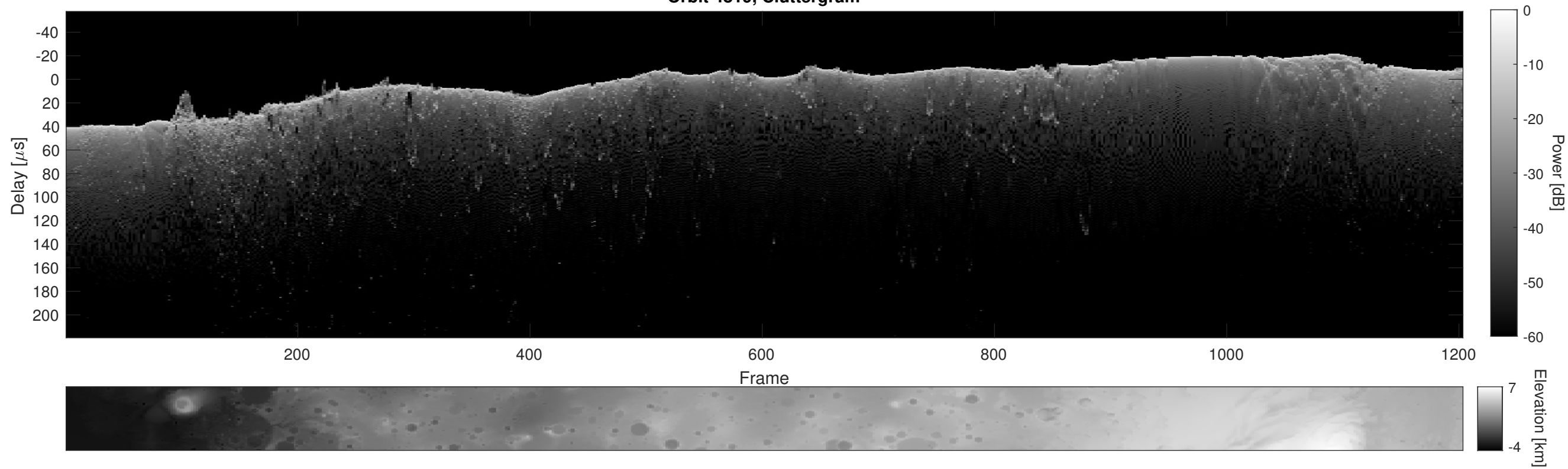
Orbit 4819, Cluttergram
