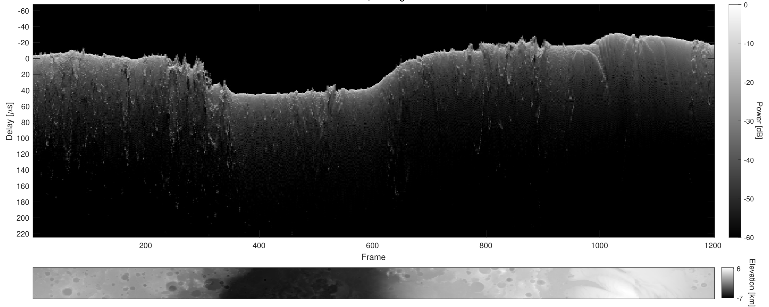
Orbit 4820, Cluttergram
