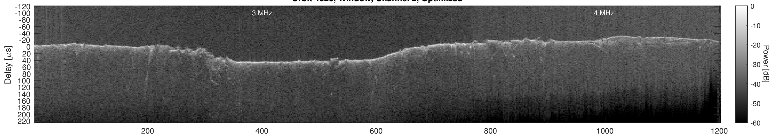
Orbit 4820, Cluttergram
