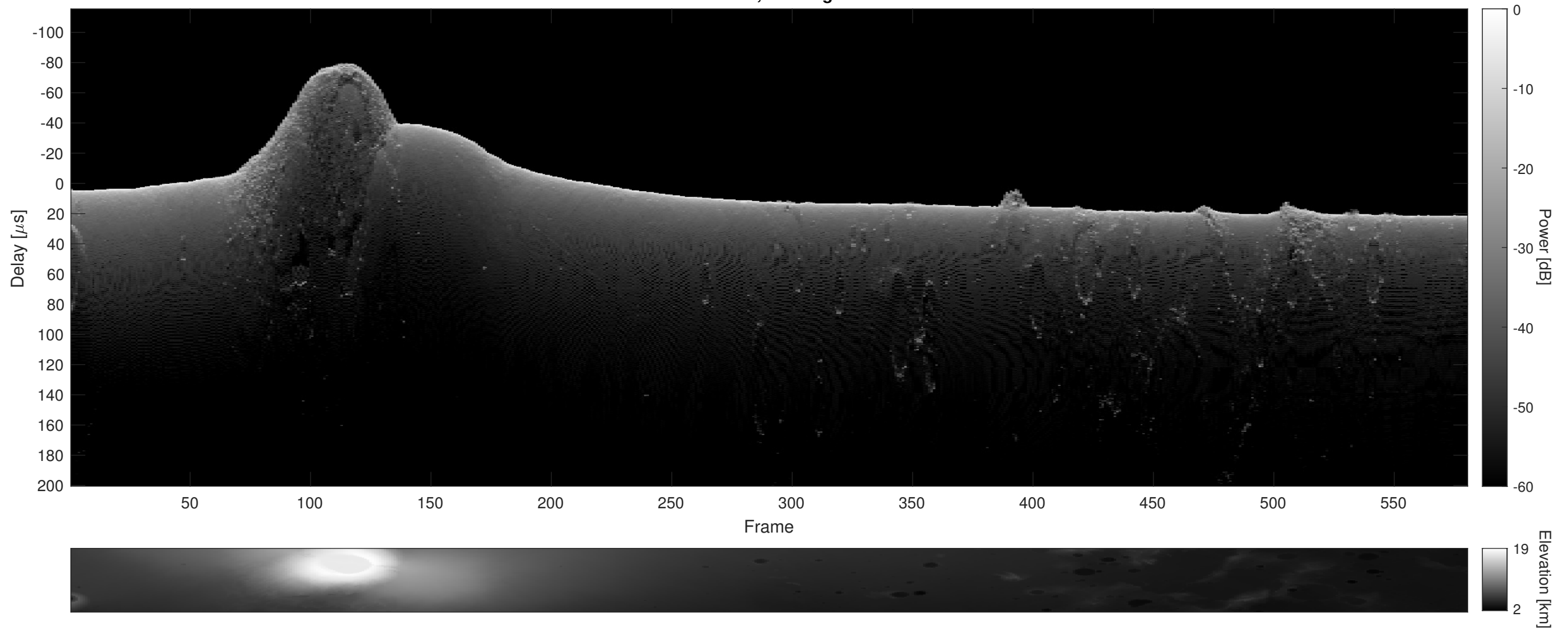
Orbit 4822, Cluttergram
