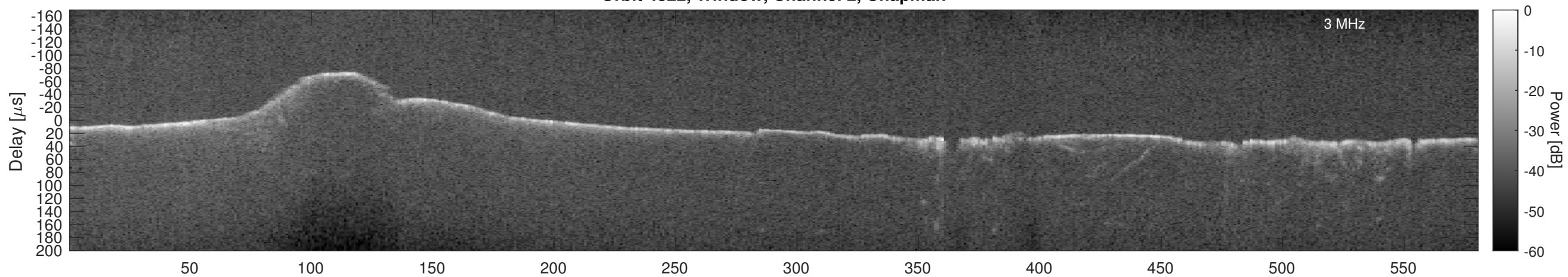
Orbit 4822, Window, Channel 2, Optimized
