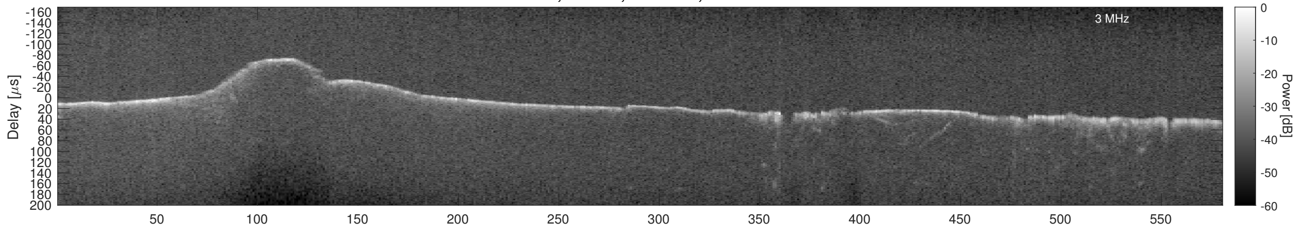
Orbit 4822, Window, Channel 2, Chapman
