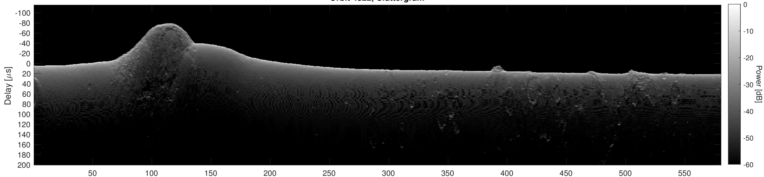
Orbit 4822, Cluttergram
