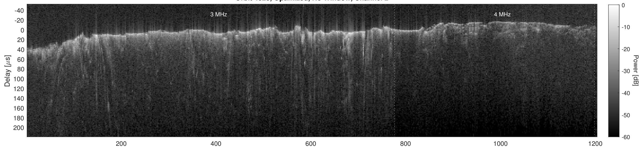
Orbit 4823, Cluttergram
