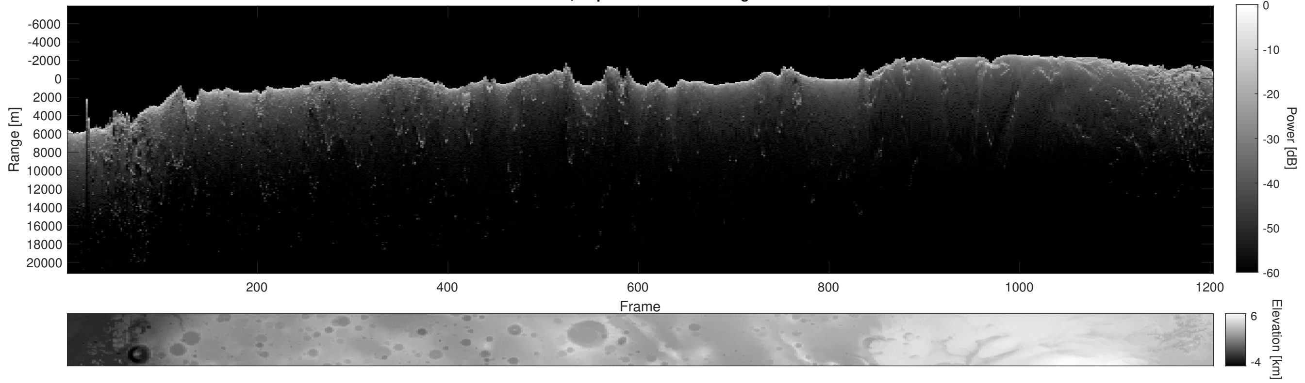
Orbit 4823, Depth-Corrected Cluttergram
