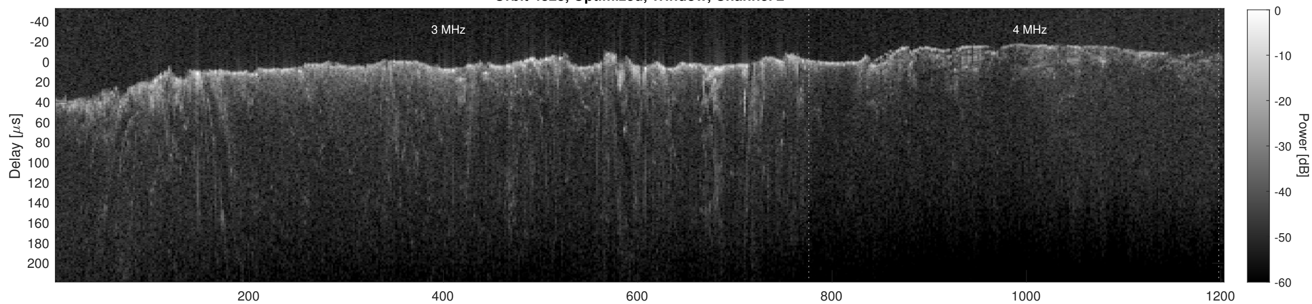
Orbit 4823, Cluttergram
