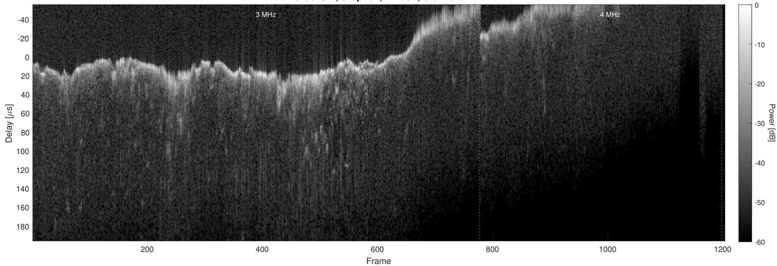
Orbit 4824, Chapman, Window, Channel 2
