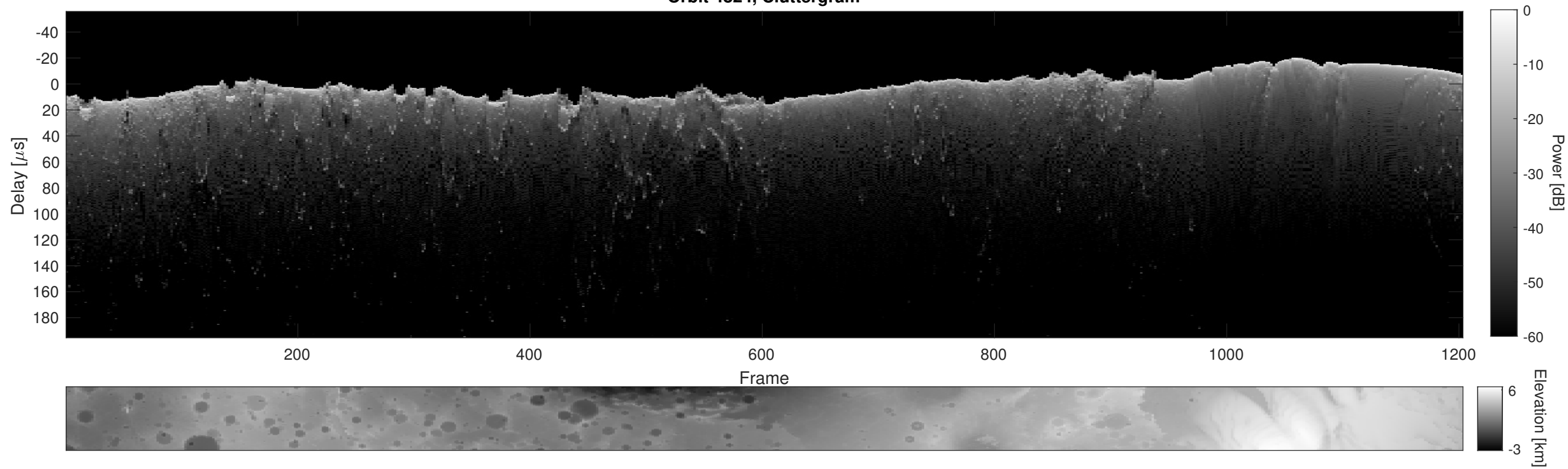
Orbit 4824, Cluttergram
