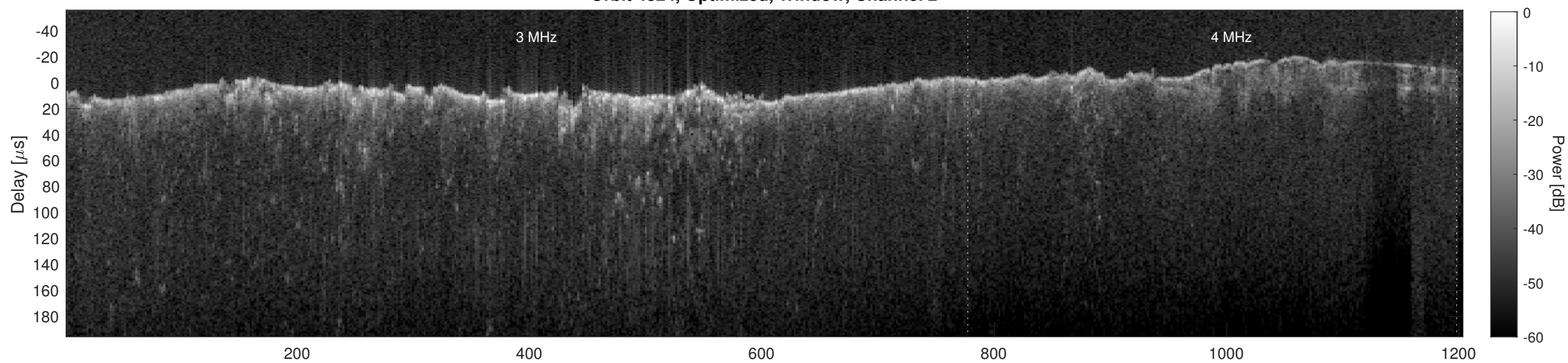
Orbit 4824, Cluttergram
