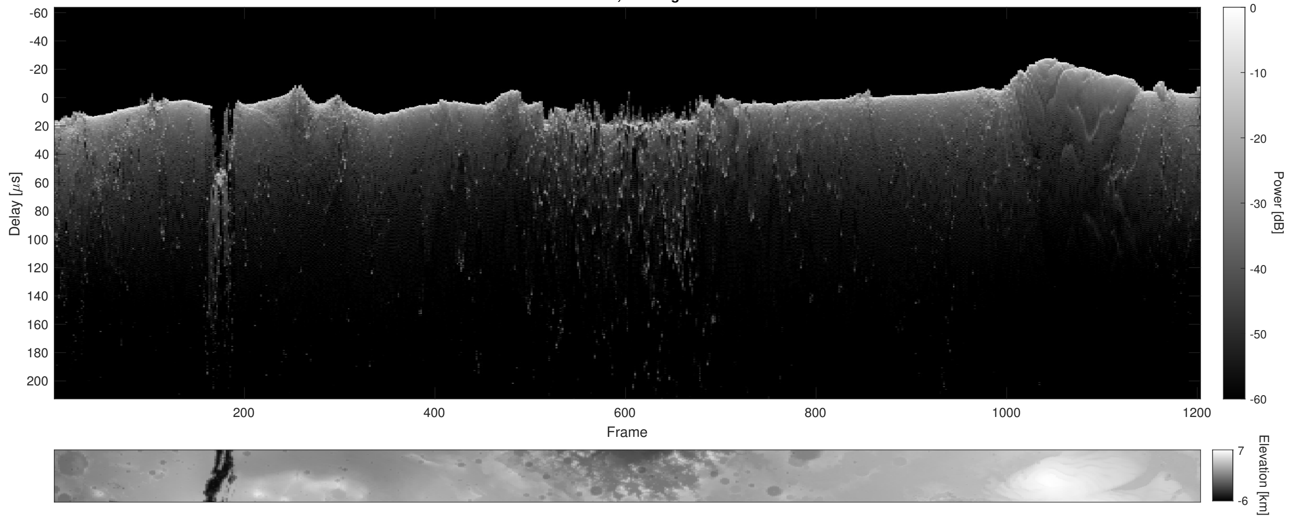
Orbit 4825, Cluttergram
