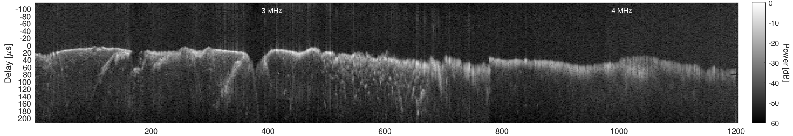
Orbit 4825, Window, Channel 2, Chapman
