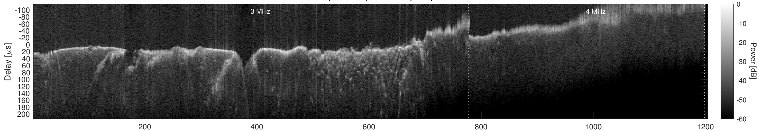
Orbit 4825, Window, Channel 2, Optimized
