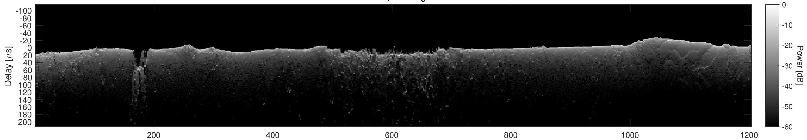
Orbit 4825, Cluttergram
