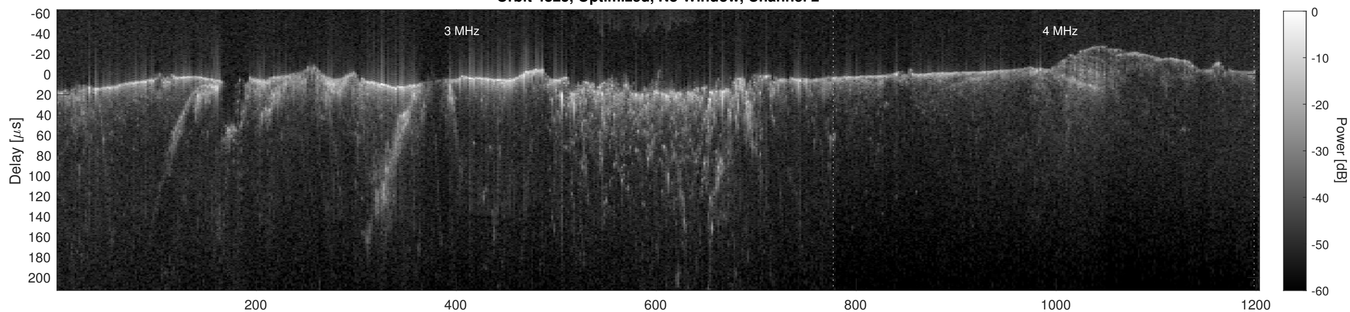
Orbit 4825, Cluttergram
