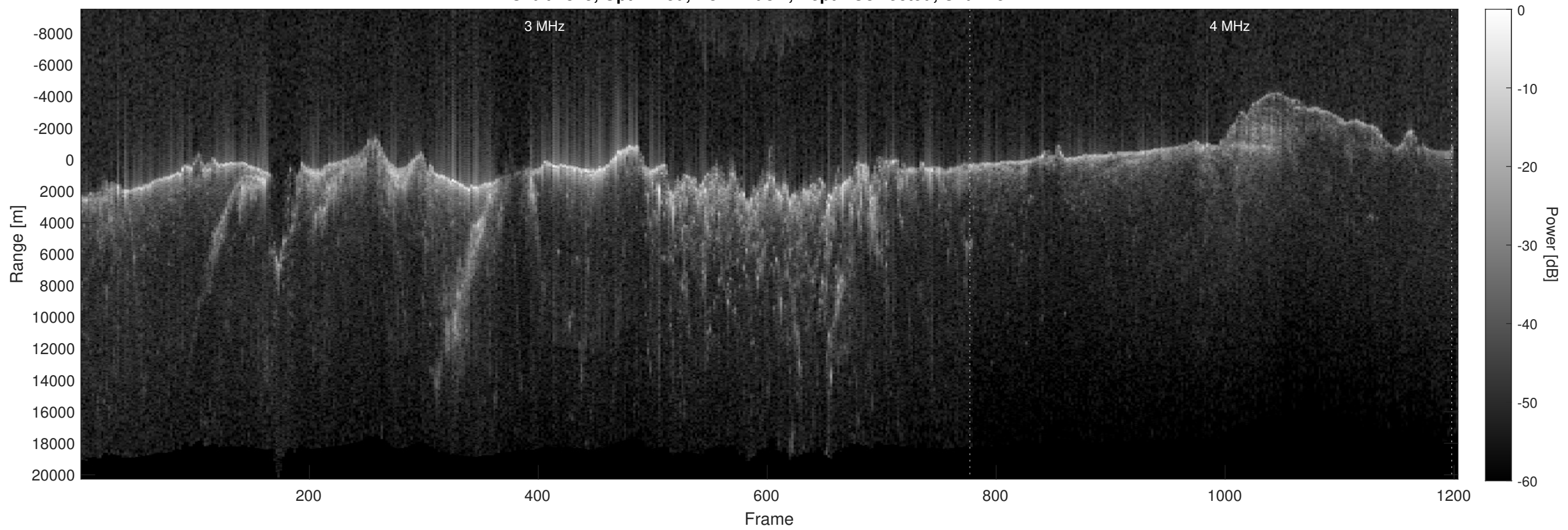
Orbit 4825, Optimized, No Window, Depth-Corrected, Channel 2
