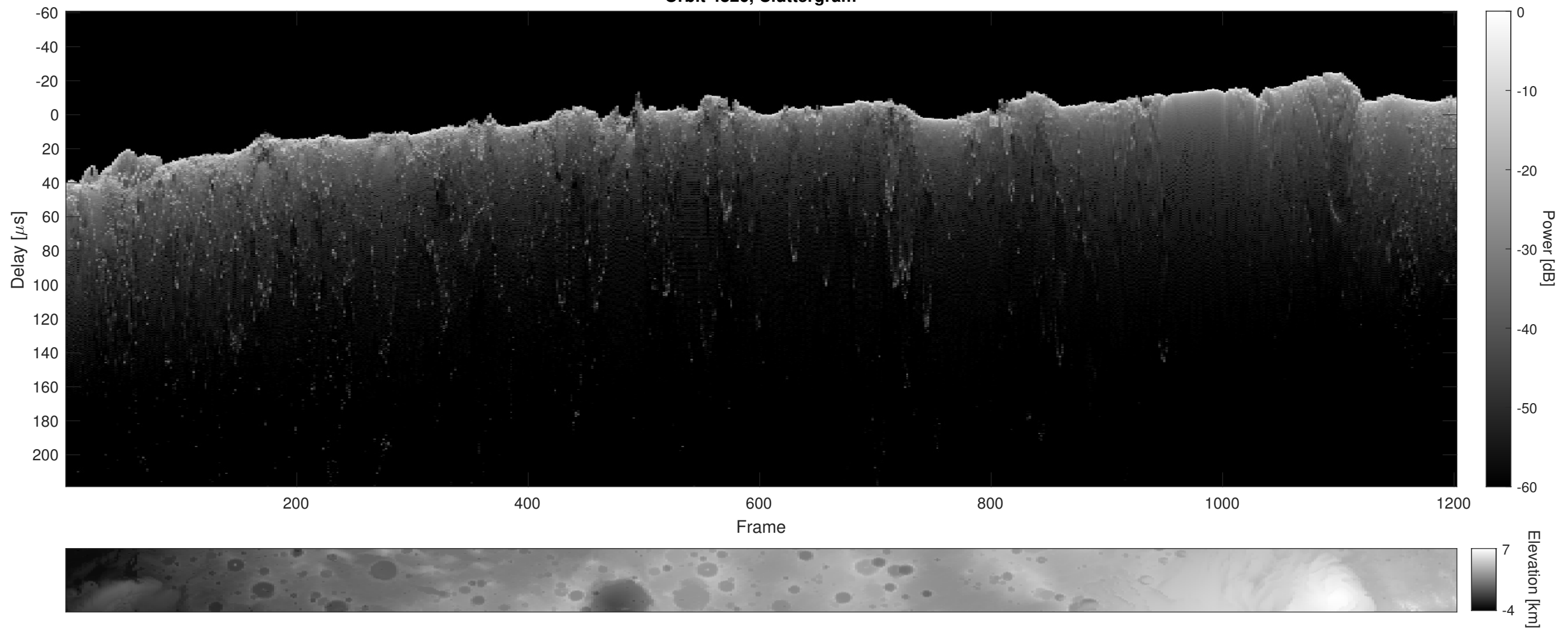
Orbit 4826, Cluttergram
