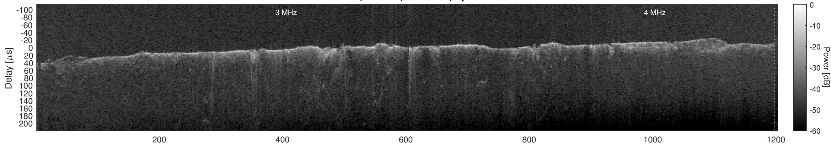
Orbit 4826, Cluttergram
