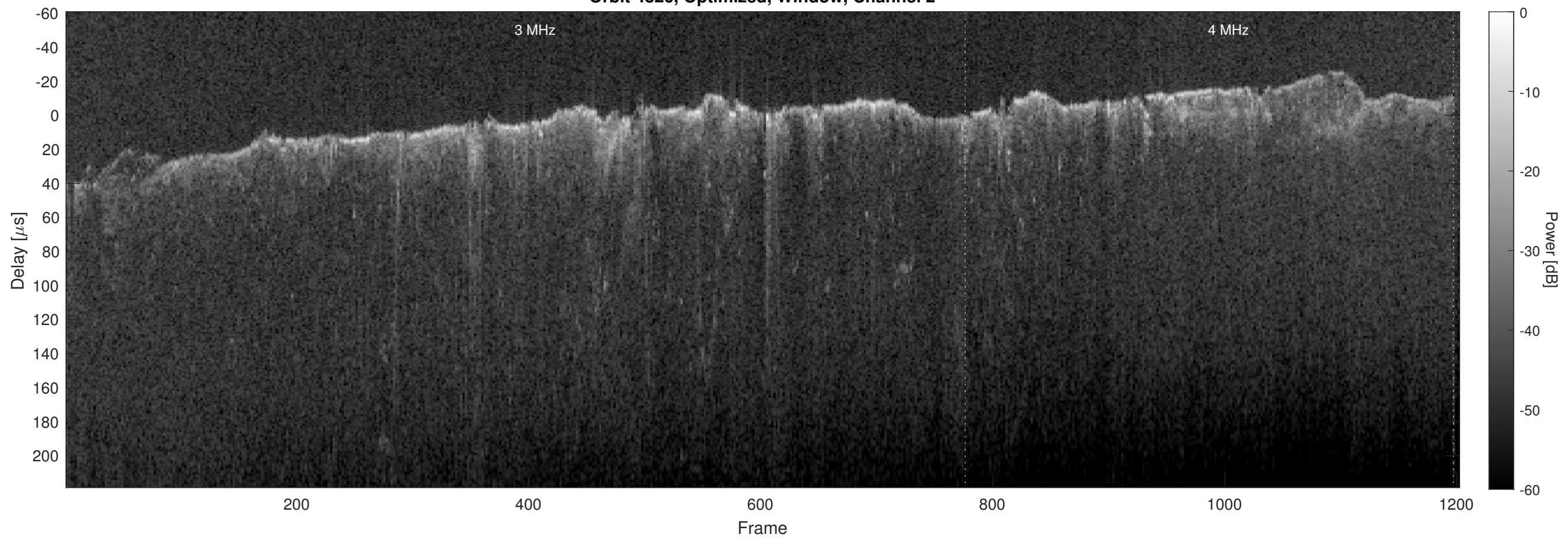
Orbit 4826, Optimized, Window, Channel 2
